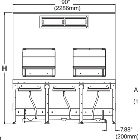
Front View – ITS3250SG-90 (without carts in bays) ITS1700SG has no sliding window
