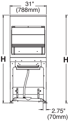
Front View ITS700SG-31 (without cart in bay) ITS500NS has sliding window only
