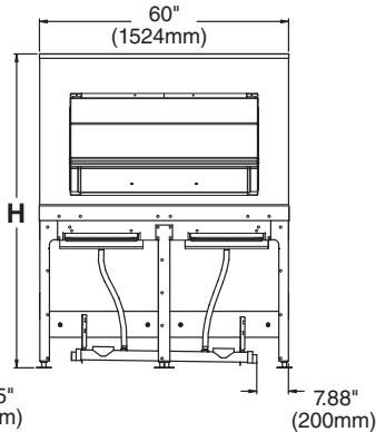
Front View ITS1350SG-60 (without carts in bays) ITS2250SG has sliding window at top of bin
